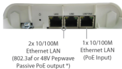
Connector Panel (Inside the Lid)
